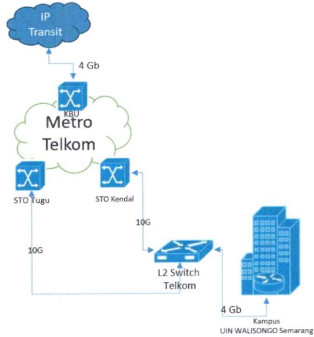
TOPOLOGI IP TRANSIT UIN WALISONGO SEMARANG
